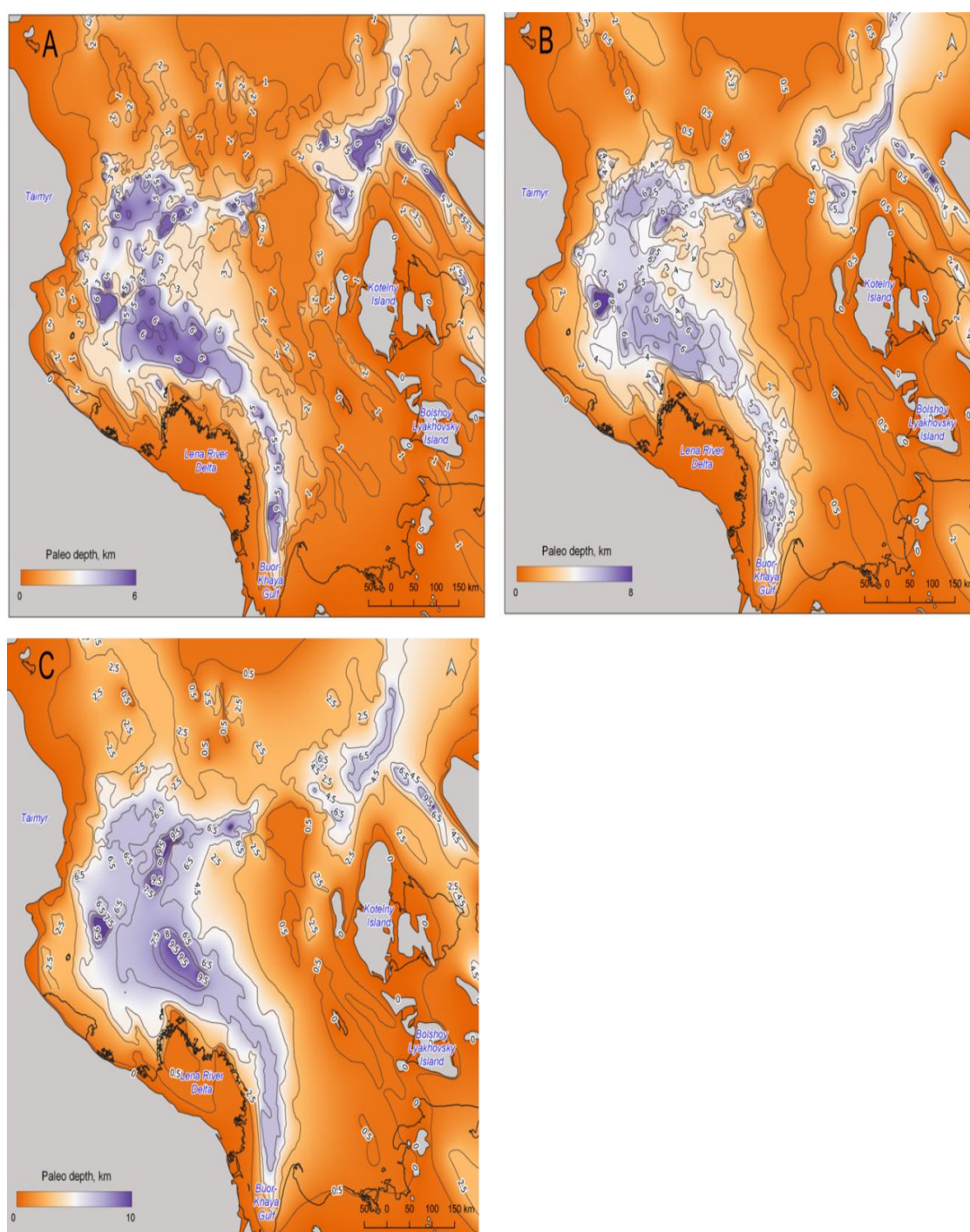
Figure 6 – Results of back-stripping analysis illustrate the base of the sedimentary cover structure at three different periods: A) at the end of the Cretaceous, B) at the end of the Eocene and C) at the beginning of the Miocene.
