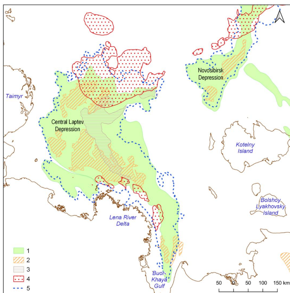
Figure 8 – Locations of the main depocentres and domains of consistent subsidence include the Central Laptev and Novosibirsk Depressions
