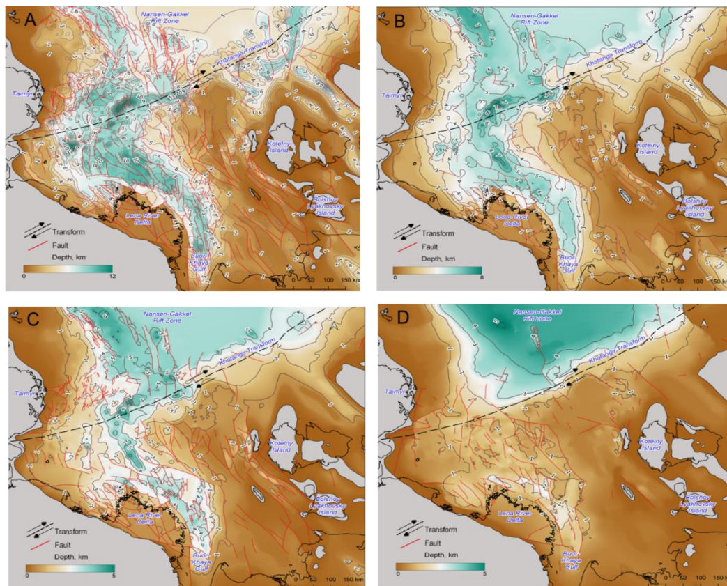
Figure 5 – Depth structure maps of the main unconformities in the sedimentary cover of the Laptev Sea: A) Pre-Aptian unconformity at the base of the Laptev Sea sedimentary cover shows a major curvilinear subsided zone in the central part. The zone is intensely faulted and consists of multiple small depressions of varied shape and orientation. The area near the New Siberian Islands and Lyakhovsky Islands hosts an uplifted zone with minor narrow depressions controlled by a system of strike-slips. A system of normal faults controls subsided zones in the northern part of the territory. B) The top Cretaceous unconformity (mBu) in the Laptev Sea shows an inherited structural pattern of the underlying pre-Aptian unconformity (A) with gentler topography. C) Top Eocene unconformity (UB) in the Laptev Sea illustrates changes in structural geometry compared to the underlying surface. These changes led to the fragmentation of the central curvilinear depression and the development of an extensive depression in the north. D) Base Miocene unconformity (RU) in the Laptev Sea shows the only sizable depression in the north of the study area and a system of shallow depressions rimming the Lena River Delta.
