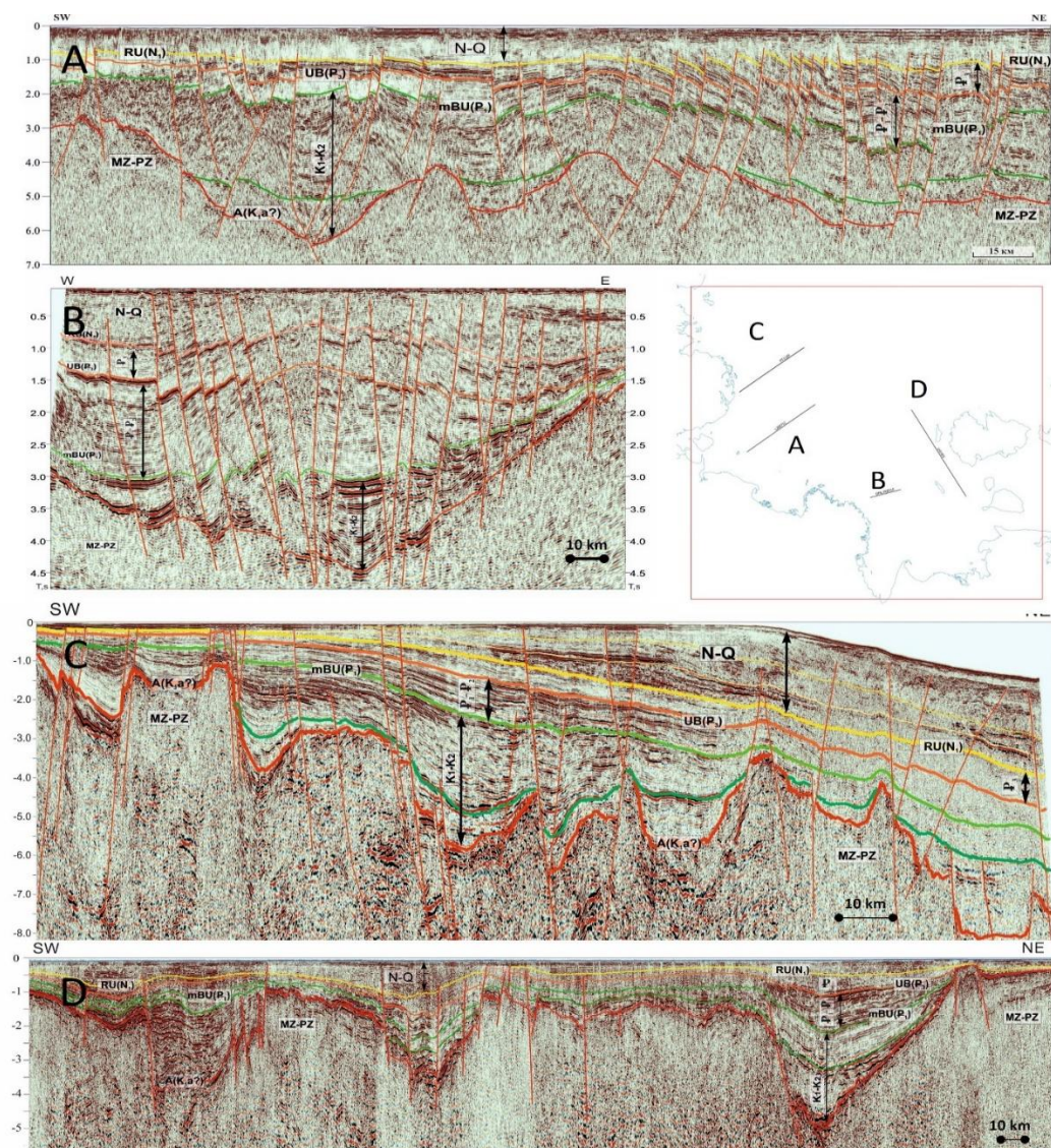
Figure 4 – Examples of different time sections are as follows: A) along the line L200712 and B) along the line OML192D10, which illustrate the complex shear nature of the Central Laptev (these sections were revised after the "MAGE" [2007] technical report and again after the RosGeo [2021] technical report); C) along the line PT1129, showcasing the extensional tectonics of the Pritaimyr area (it was revised after the "MAGE" [2013] technical report); D) along the line LH1401, providing insights into the geology of the Eastern Laptev and revealing mostly lower thicknesses of sedimentary cover with a few small grabens (this section was revised after the "MAGE" (2014) technical report
