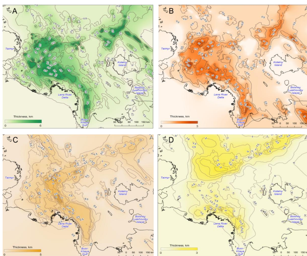
Figure 7 – Isopach maps represent the thickness of the main sedimentary units.
